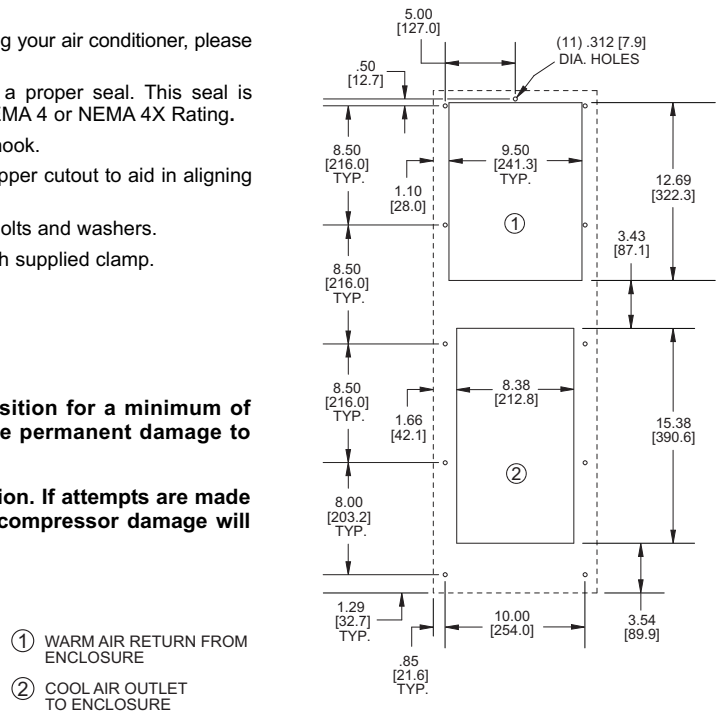
MOUNTING PLAN
