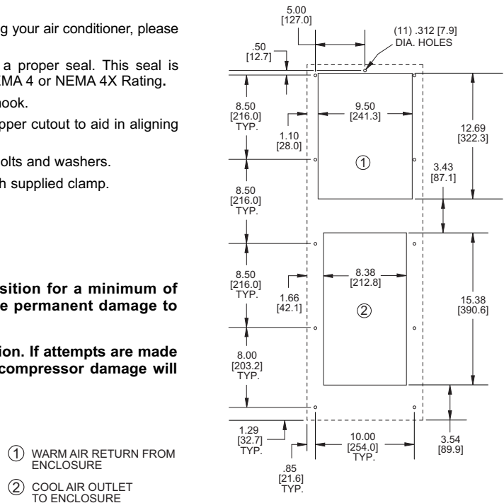
MOUNTING PLAN
