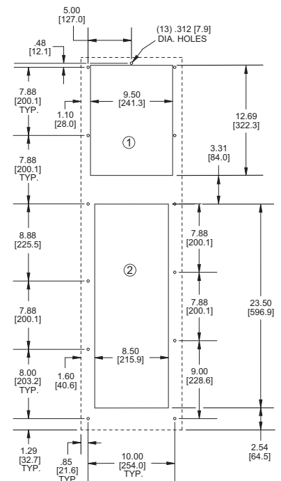
MOUNTING PLAN
