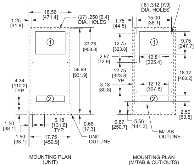
MOUNTING PLAN
