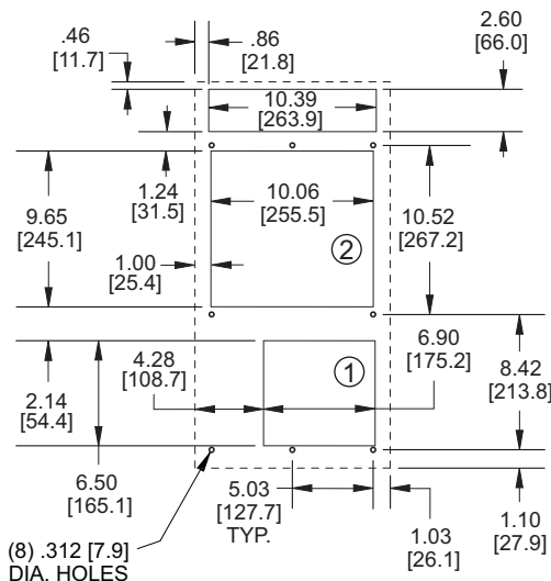
MOUNTING PLAN
