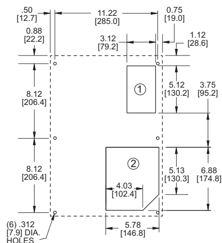
NEMA 12 MOUNTING PLAN
