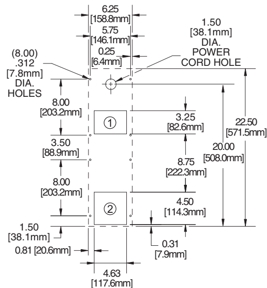
MOUNTING PLAN
