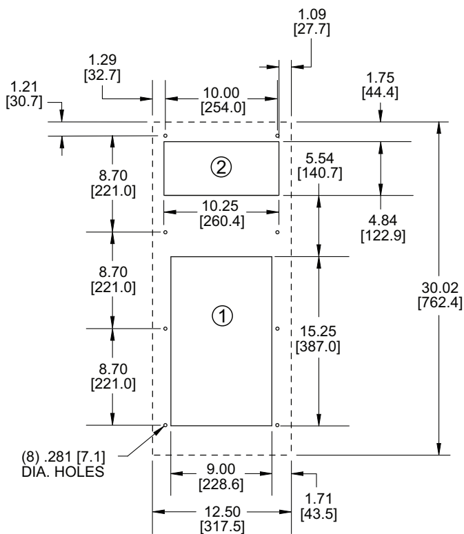
MOUNTING PLAN
