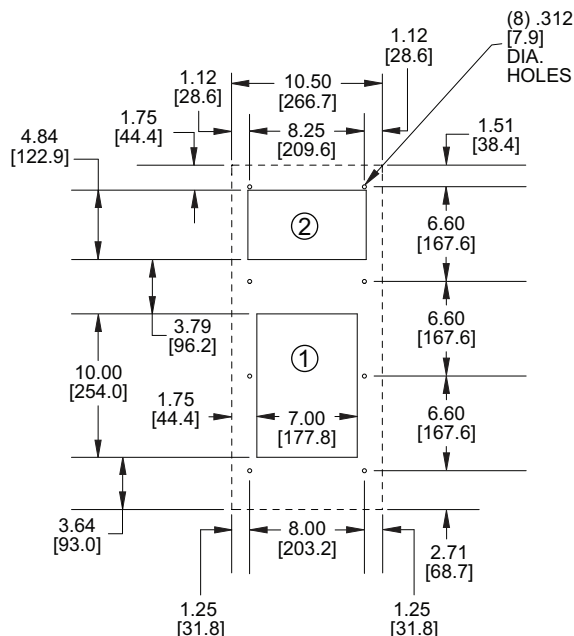
MOUNTING PLAN
