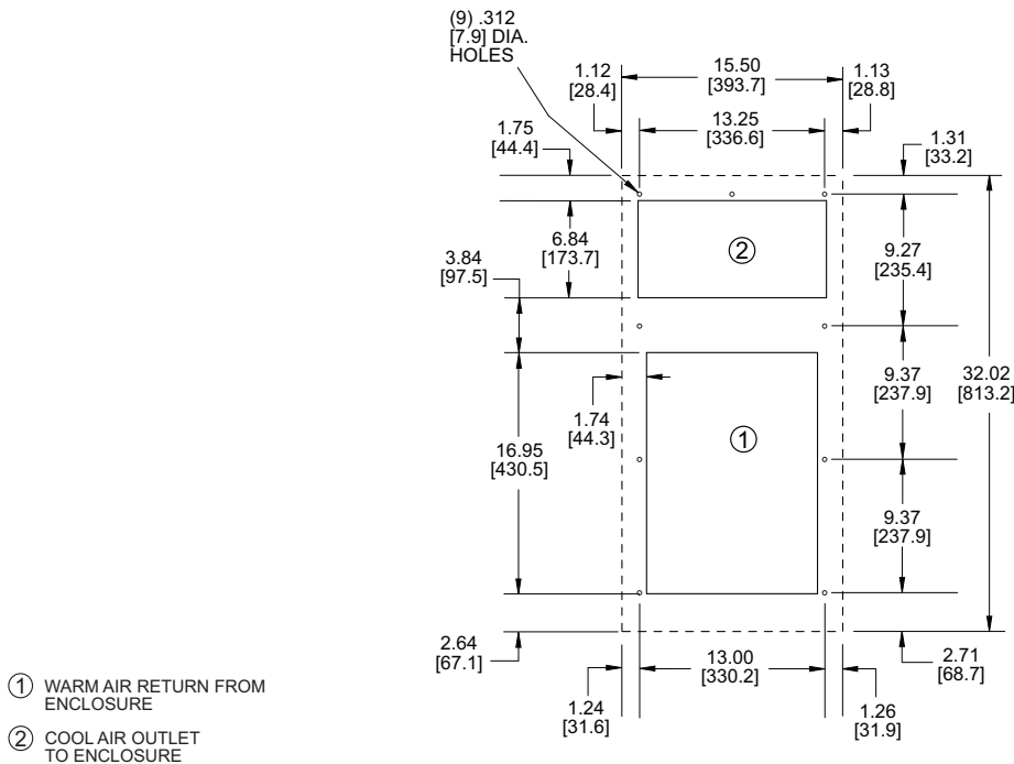
MOUNTING PLAN
