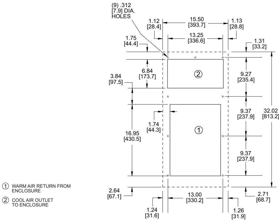
MOUNTING PLAN
