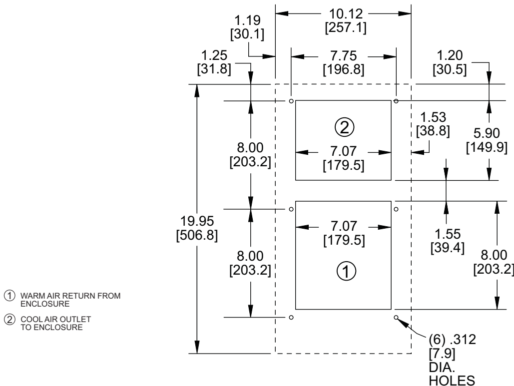
MOUNTING PLAN
