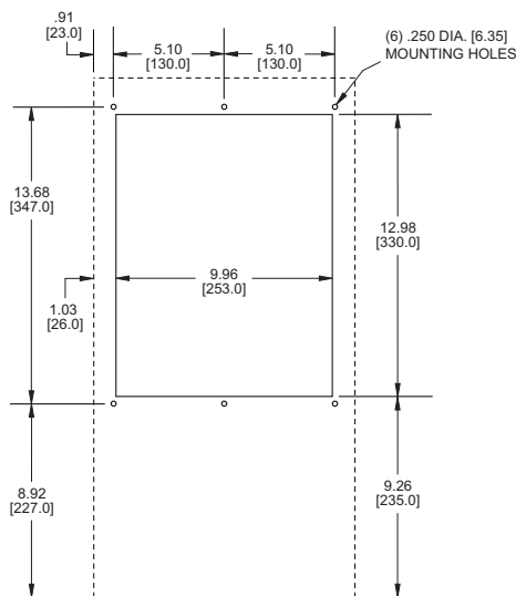
MOUNTING PLAN
