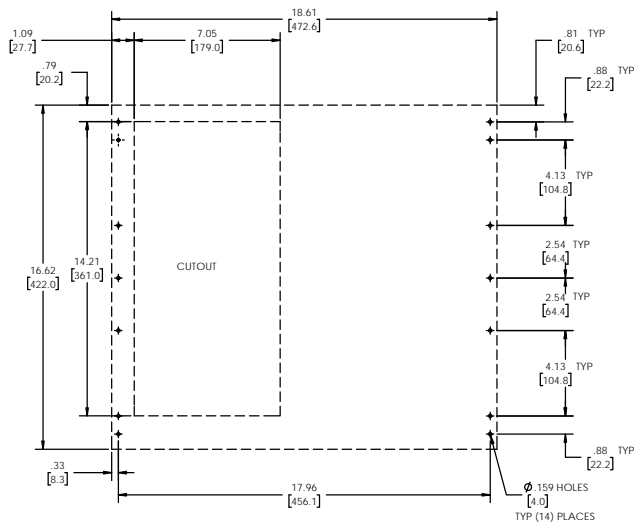
MOUNTING PLAN: FRONT PANEL WITH L-BRACKETS
