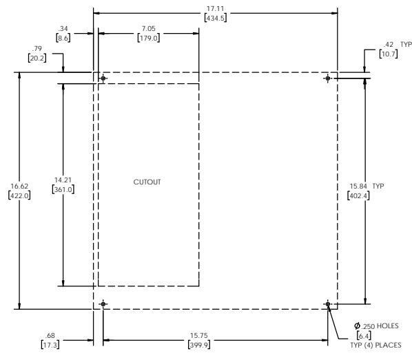
MOUNTING PLAN: FRONT PANEL WITH RIVNUTS
