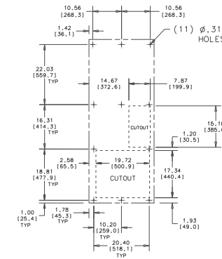
MOUNTING PLAN
