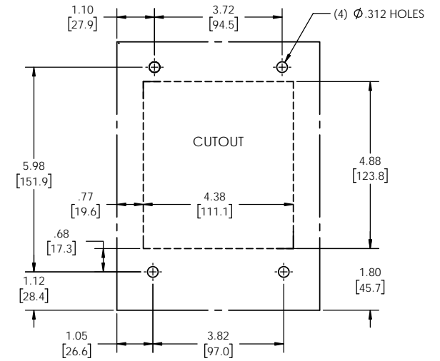
MOUNTING PLAN
