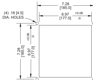
MOUNTING PLAN
