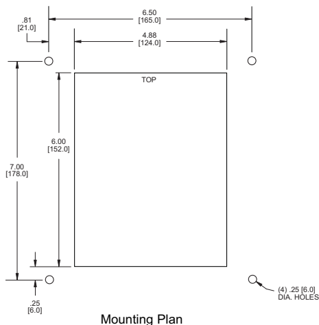
Mounting Plan
