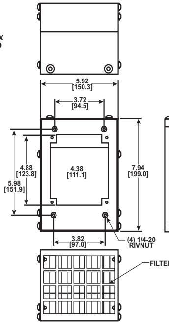
MOUNTING PLAN
