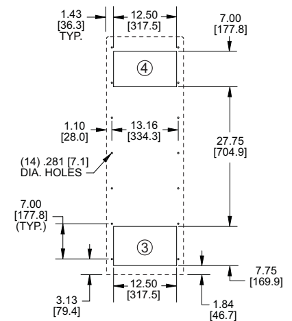
MOUNTING PLAN
