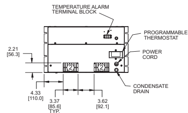
MOUNTING PLAN
