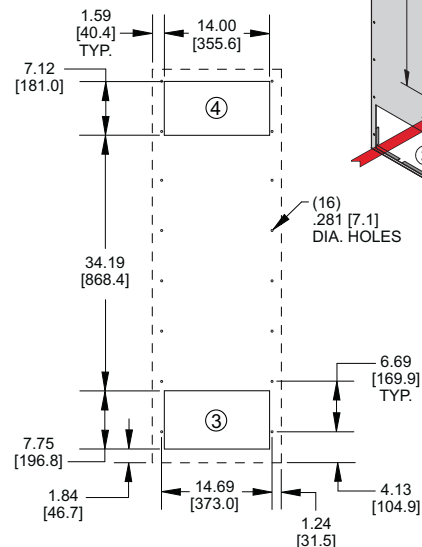
MOUNTING PLAN
